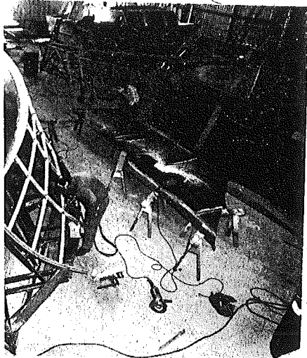
U-welded aluminium-hulled diesel engine fabricated on a rolling cradle by the latest submerged-arc welding
